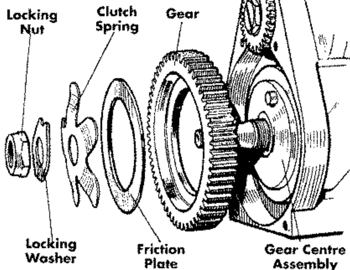
Mail Magneto Gear Kit (incl. dynamo Drive Gear) Genuine Lucas £ 35.00 (Parts sold separate)
